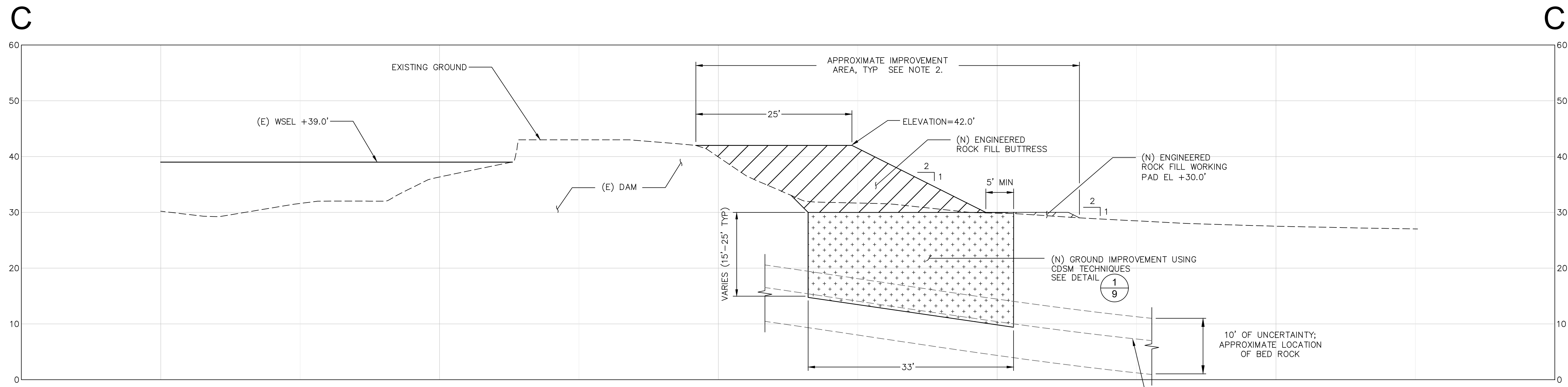
C 8 SECTION (THRU NORTH DAM) SCALE: 1"=10'
