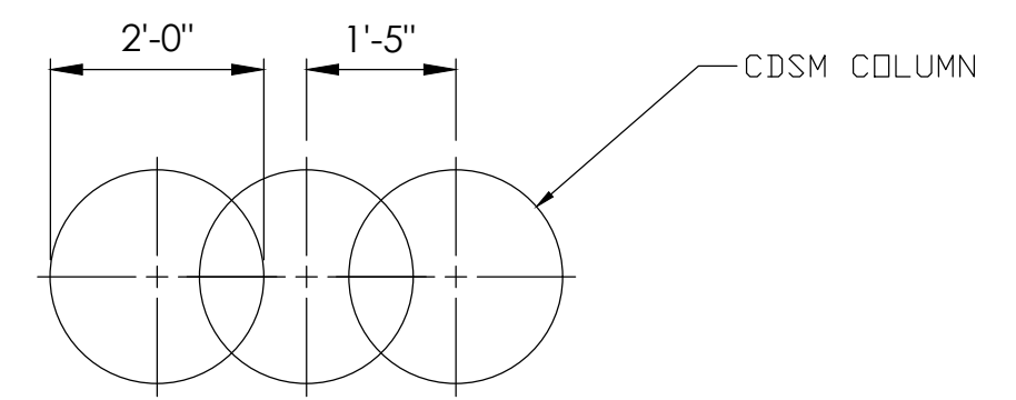
CDSM COLUMN DIAMETER & SPACING DETAIL, TYP SCALE: 1"=2'
