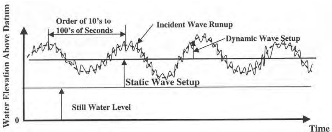
Figure 1 Definitions of Static and Dynamic Wave Setup and Incident Wave Runup. Reproduced from [04].
