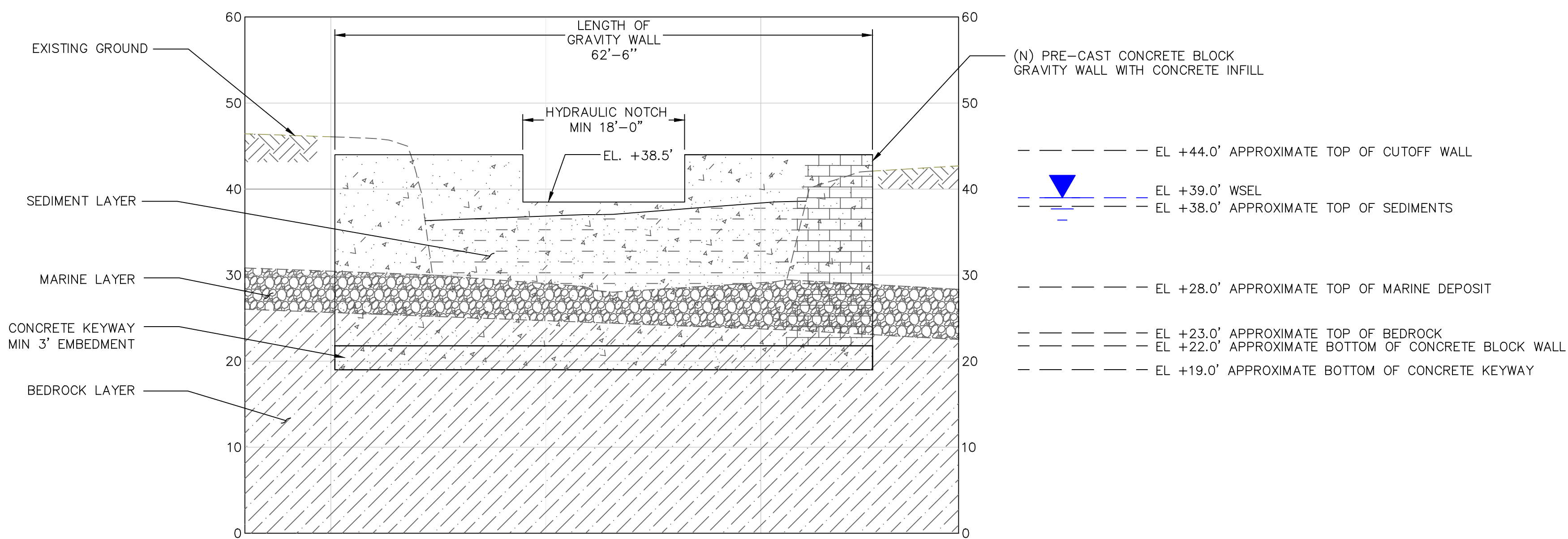
1 10 GRAVITY WALL PLAN SCALE: 1"=10'
