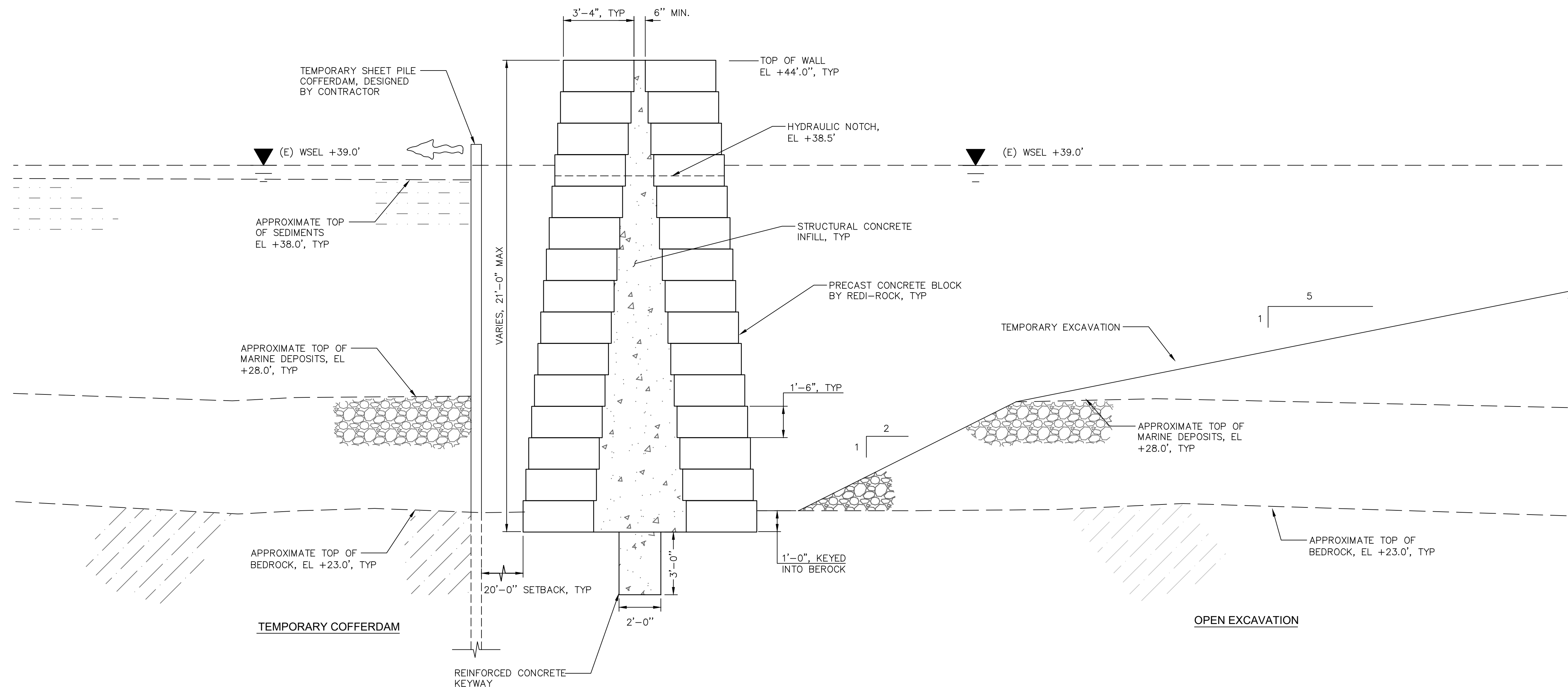
B 10 GRAVITY WALL SECTION NTS
